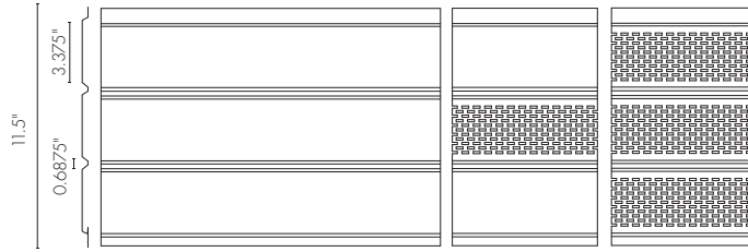
12" TruLine® HP Soffit
