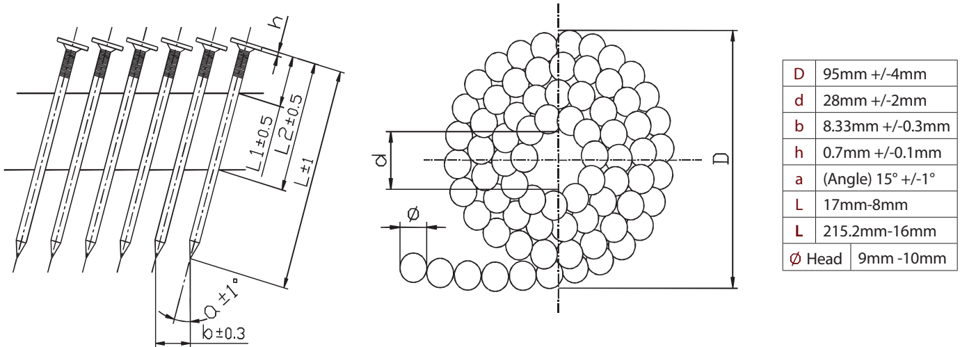
ASTM F 1667-05 Table 29 Type 1, Style 20 - Roofing Nails
